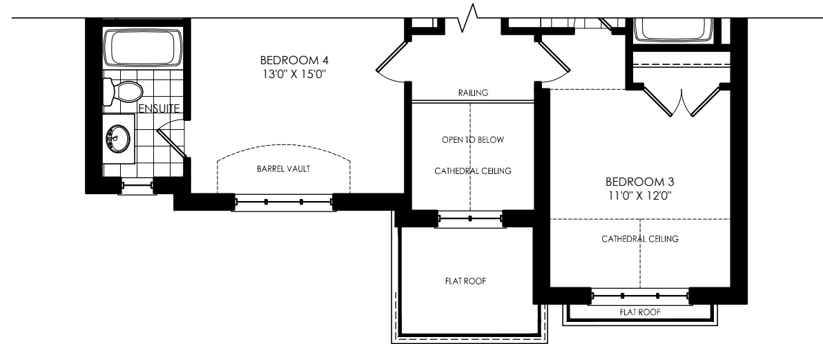
PARTIAL SECOND FLOOR PLAN ELEV 'B'
