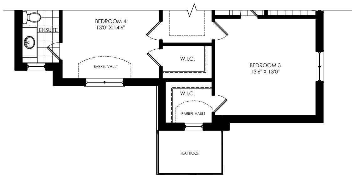
PARTIAL SECOND FLOOR PLAN ELEV 'B'
